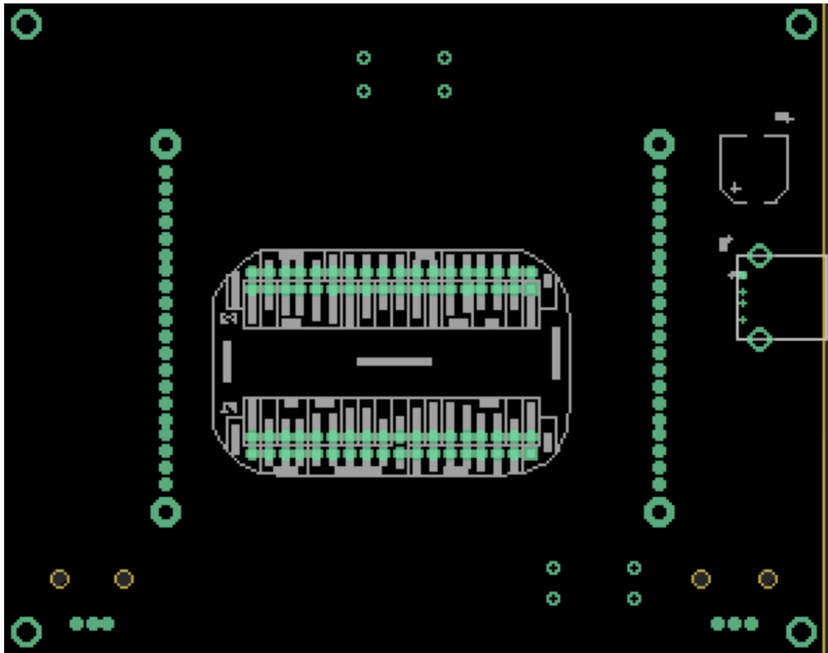
Back Layer Photo of Etch a Sketch PCB
